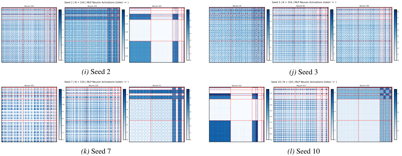
Figure 19. MLP feature stability across seeds and moduli. Each subplot shows activation maps of three randomly sampled MLP neurons, reordered according to the \mathcal{J} -class decomposition of \mathbb{Z}_n . Across seeds and moduli, we observe consistent emergence of block-structured activations aligned with multiplicative \mathcal{J} -classes, indicating that the learned representation is stable across random initializations.
